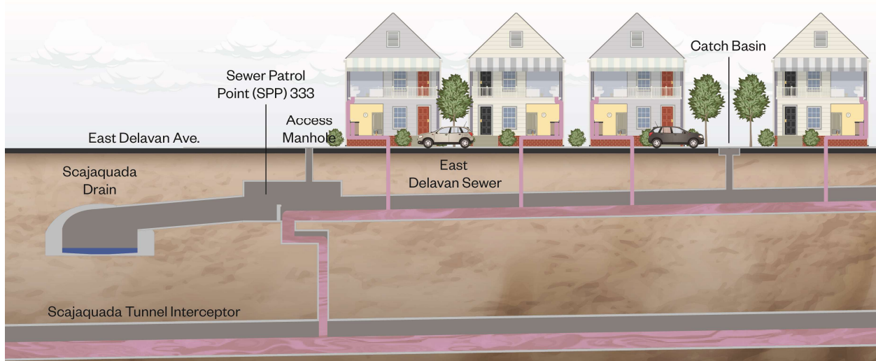
Figure 3-11: Existing Dry Weather Flow Conditions
