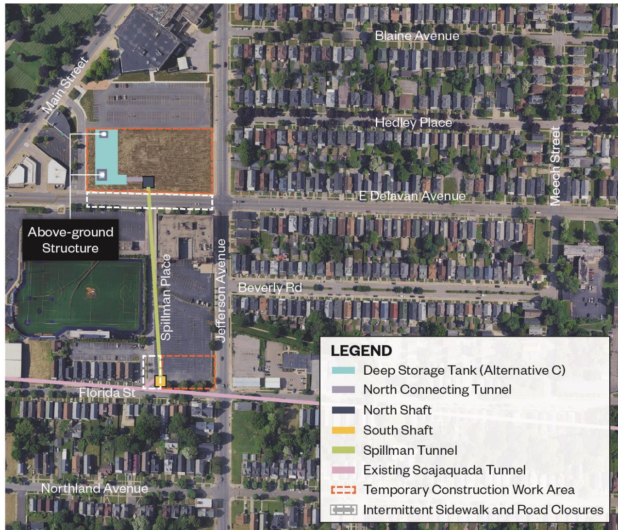
Figure 2-2: Deep Storage Tank (Alternative C) Construction Areas
