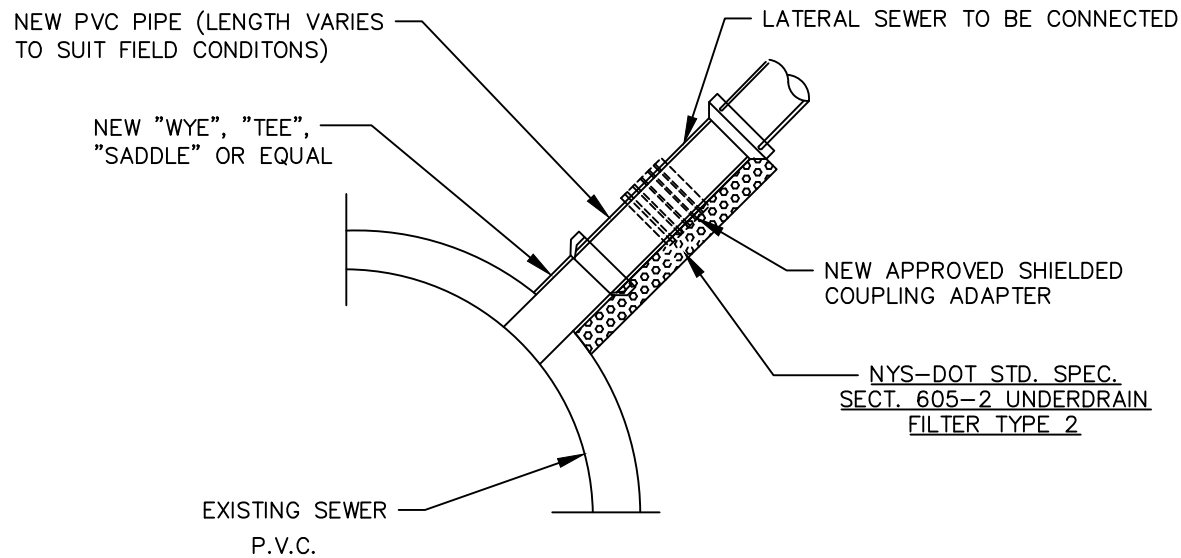
DETAIL TYPICAL NEW LATERAL CONNECTION TO EXISTING SEWER N.T.S.
