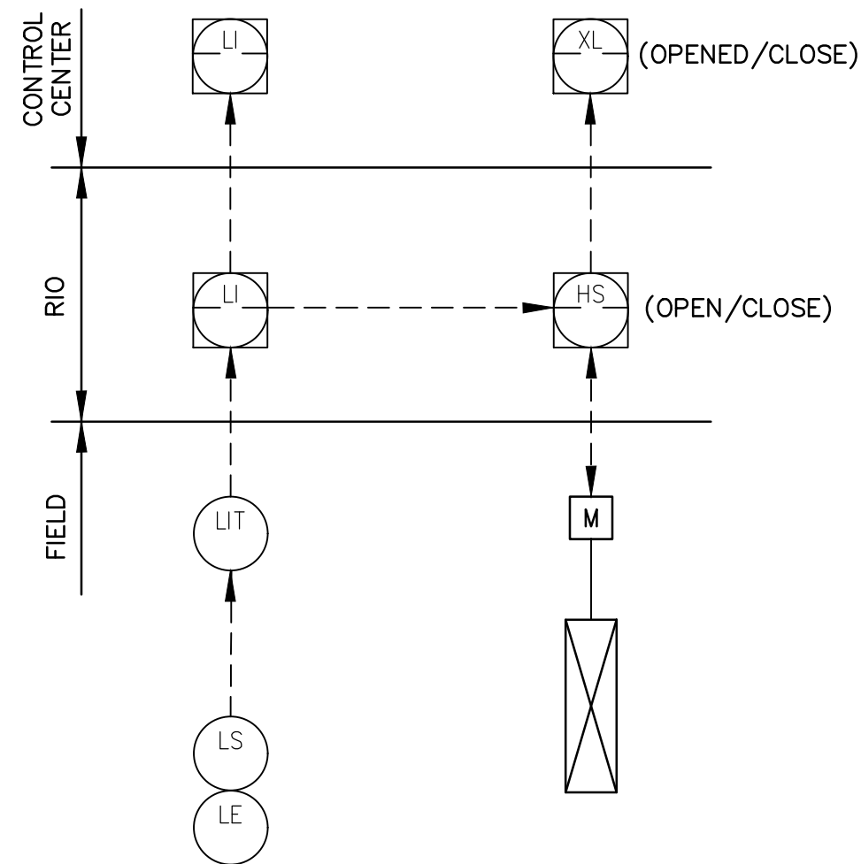
TYPICAL INSTRUMENTATION AND CONTROL DETAIL
