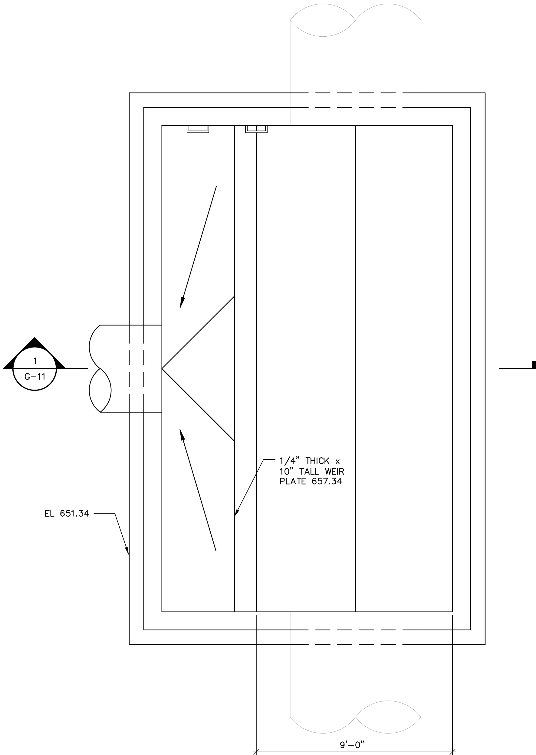
SECTIONAL PLAN SCALE: 3/8" = 1'-0"
